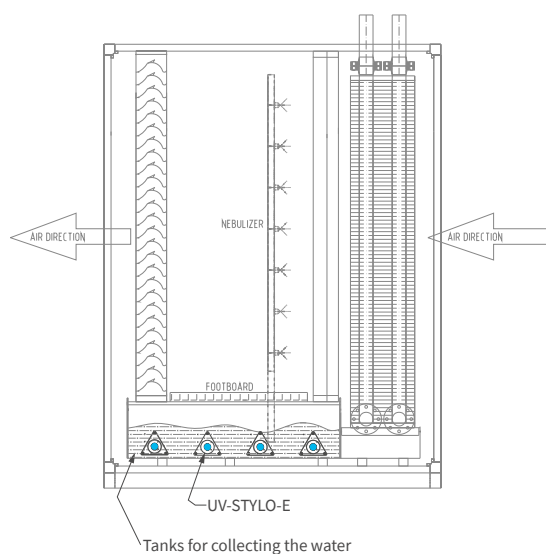
Application scheme
